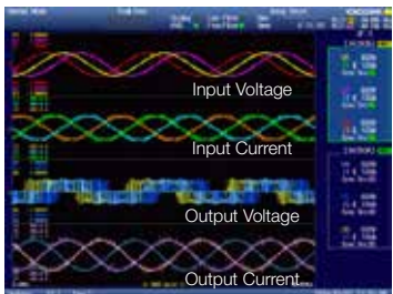
Matrix Drive Rated Power Operation
